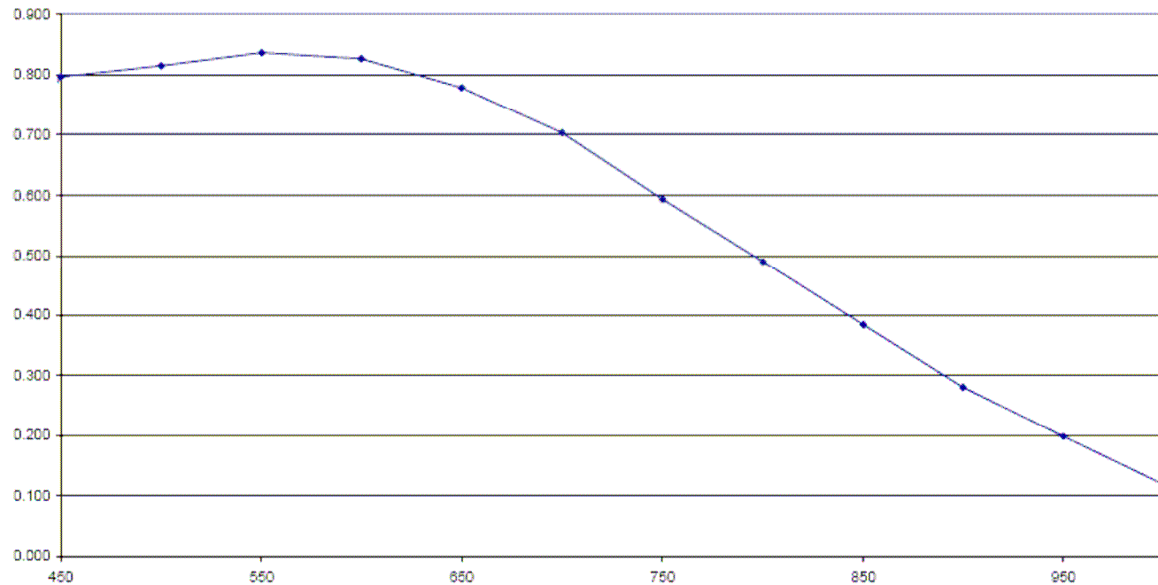
Quantum Efficiency
